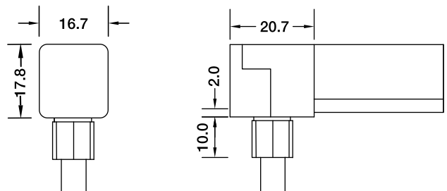
Bottom Entry Connector MJ-18-D3-B02SM MJ-18-D3-B03SFM
