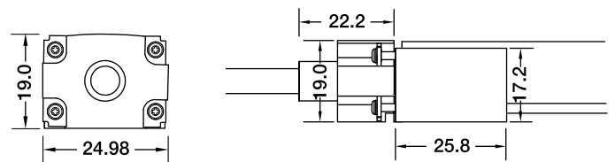
DIY Screw Connector DIY-SC-FR-16-D-01SF/02SM-D3
