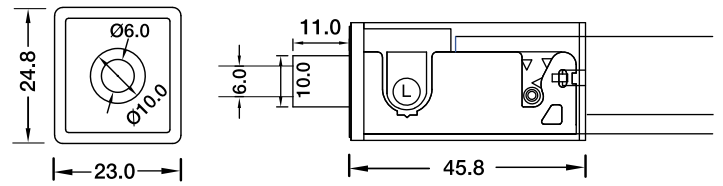
DIY Snap Connector DIY-SN-FR-16-D-01SF/02SM-D3
