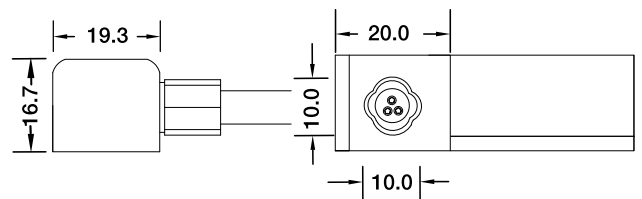
Side Entry Connector MJ-18-D3-S02SM MJ-18-D3-S03SFM
