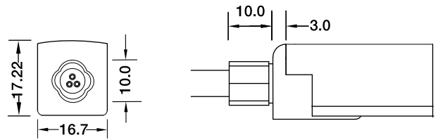
Direct Entry Connector MJ-18-D3-D02SM MJ-18-D3-D03SFM
