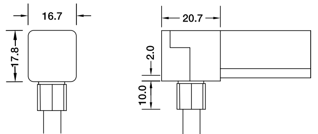
Bottom Entry Connector MJ-18-D5-B02SM MJ-18-D5-B03SFM
