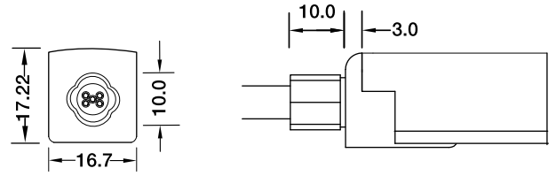
Direct Entry Connector MJ-18-D5-D02SM MJ-18-D5-D03SFM
